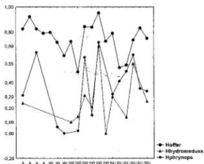
Figure 2. Seasonal variation of the H' indices for prey abundance and diet of both species studied. Abbreviations: A, autumn; SP, spring; SU, summer; W, winter.
