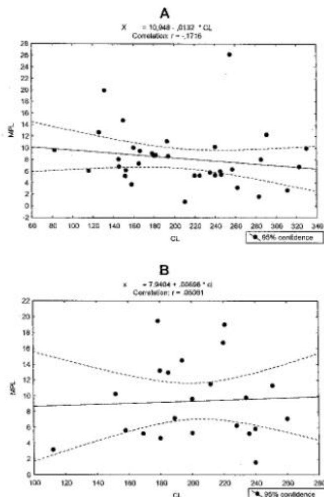
Figure 3. Pearson correlation between size of turtles (x-axis; straight-line carapace length in mm) and mean size of prey items (y-axis; mean prey length in mm) for Phrynos hilarii (A) and Hydromedusa tectifera (B).
