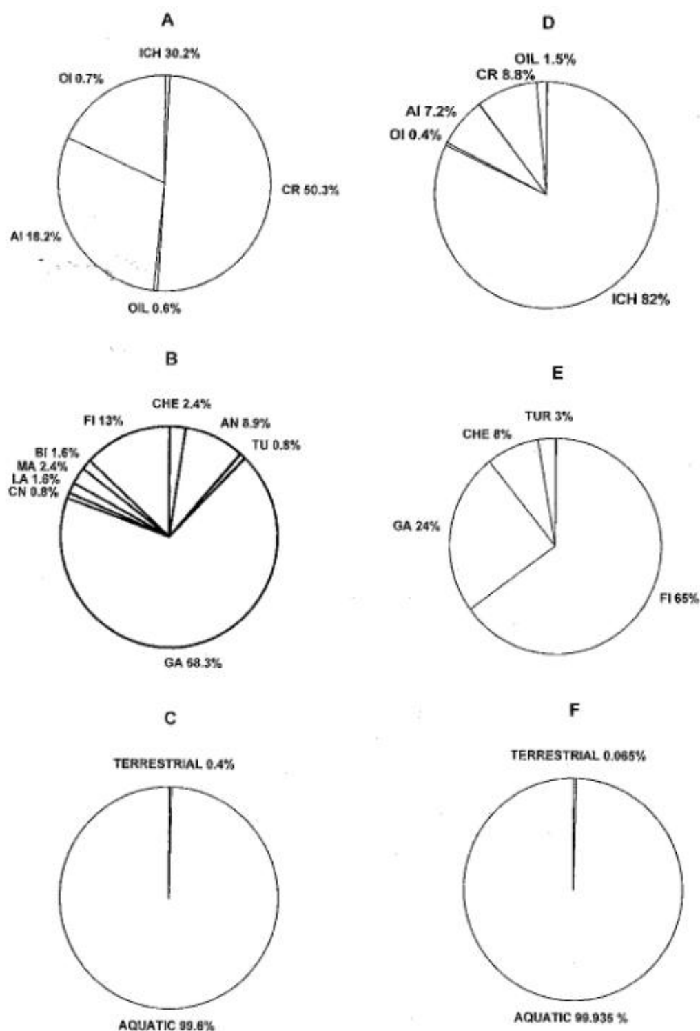
Figure 1. Pie charts showing prey category percentages for Phrynops hilarii (A–C) and Hydromedusa tectifera (D–F). A and D show the percentages of the most inclusive prey categories. B and E represent percentages of categories included within the "other" fraction shown in A and D. C and F are the percentages of terrestrial and aquatic prey items, respectively. Abbreviations: AI, adult insects; AN, annulata; BI, bird rests; CHE, chelicerata; CN, cnidaria; CR, crustacea; FI, fish; GA, gastropoda; ICH, immature chironomids; LA, larval anurans; MA, mammal rests; OI, other items; OIL, other insecta larvae; TU, turbellaria; TUR, turtle rests.
